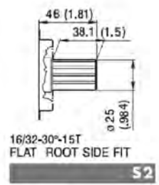
S2 16/32-30°-15T FLAT ROOT SIDE FIT Coppia Max Max Torque 660 Nm
