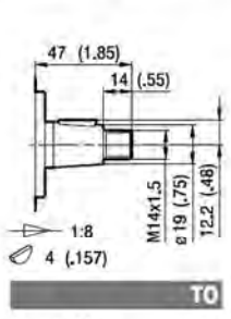
TO Coppia Max Max Torque 280 Nm
