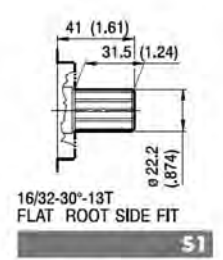
S1 16/32-30°-13T FLAT ROOT SIDE FIT Coppia Max Max Torque 405 Nm
