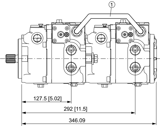
Alberi per pompe in tandem / Shafts for combination pumps
