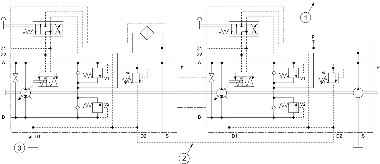
SCHEMA IDRAULICO TANDEM (TS) VERSIONE CORTA SHORT VERSION TANDEM (TS) HYDRAULIC LAYOUT
