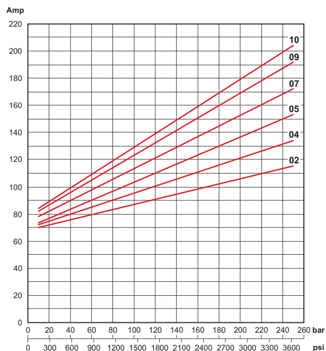
Current with GR05 / GR1 pumps Displacement 0.2 \div 1.0 \text{ cc/rev} [ 0.012 \div 0.061 \text{ in}^3/\text{rev} ]
