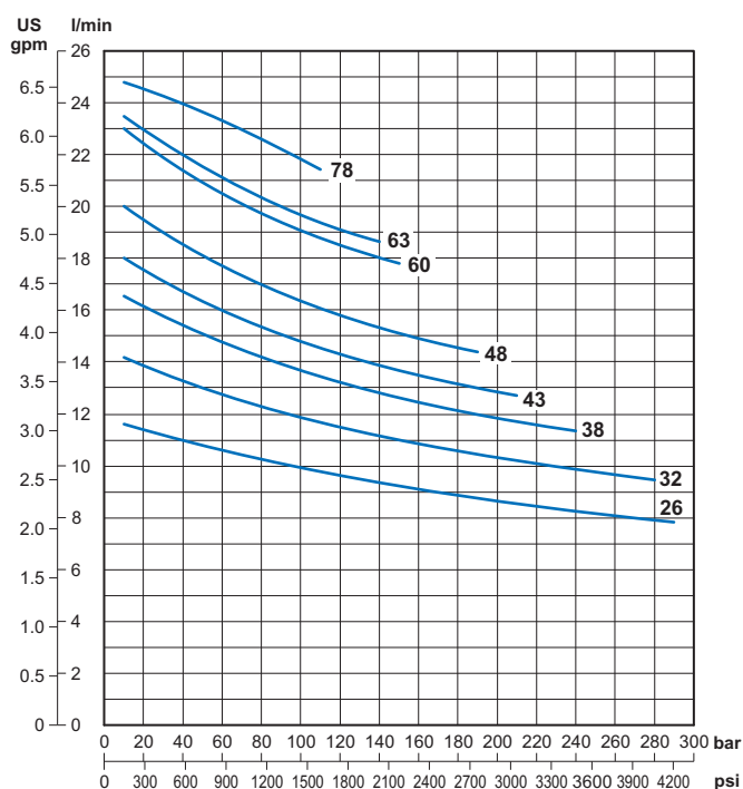
Performance with GR1 pumps Displacement 2.6 ÷ 7.8 cc/rev [0.159 ÷ 0.476 in³/rev]
