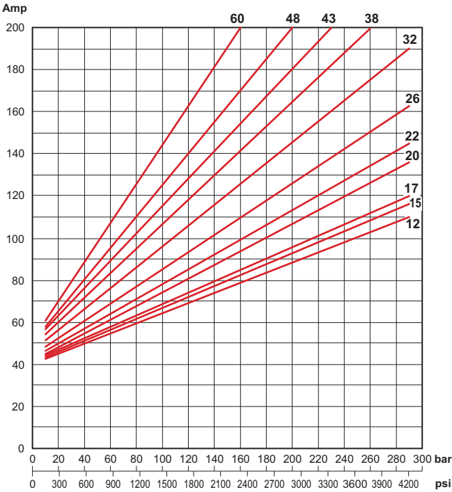
Current with GR05 / GR1 pumps Displacement 1.2 ÷ 6.0 cc/rev [0.073 ÷ 0.366 in³/rev]
