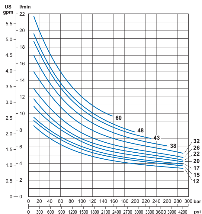
Performance with GR05 / GR1 pumps Displacement 1.2 ÷ 6.0 cc/rev [0.073 ÷ 0.366 in³/rev]
