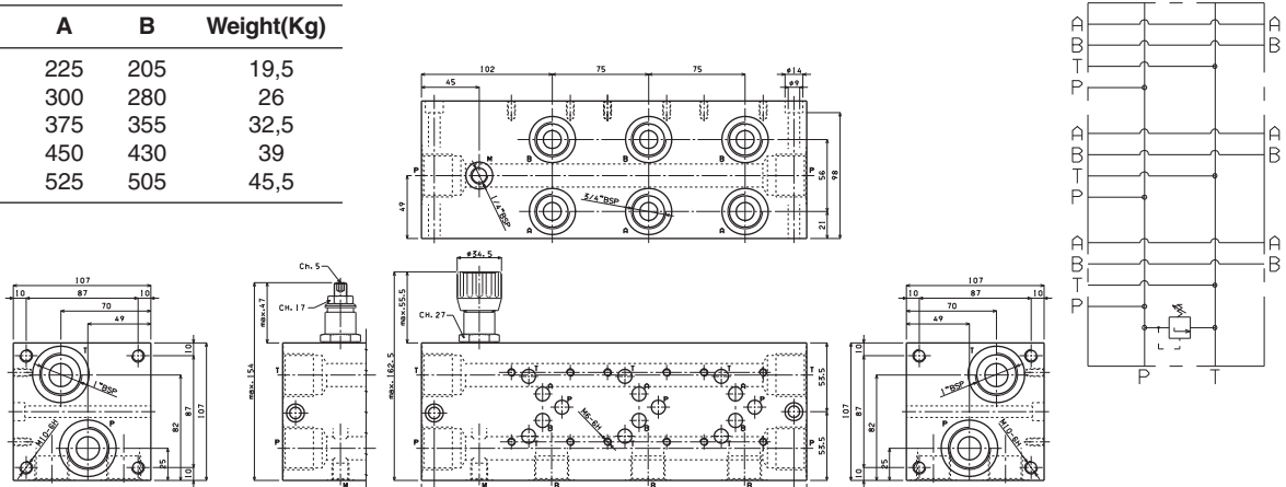
Fixing screws M8x110 UNI 5931
