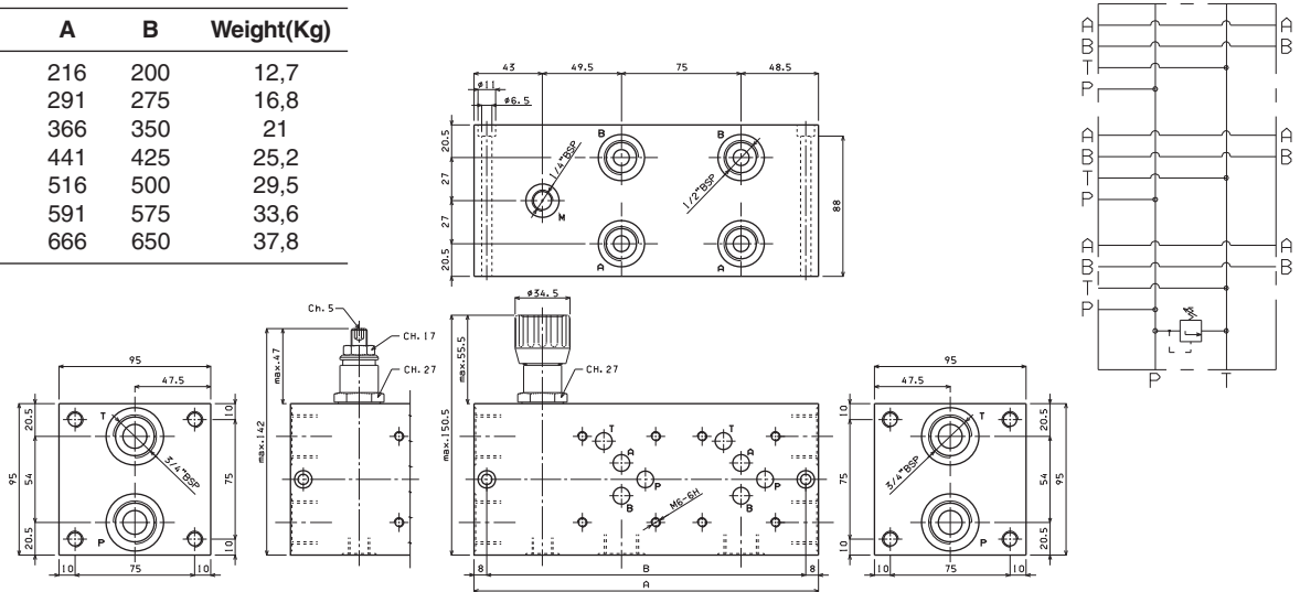
Fixing screws M6x100 UNI 5931
