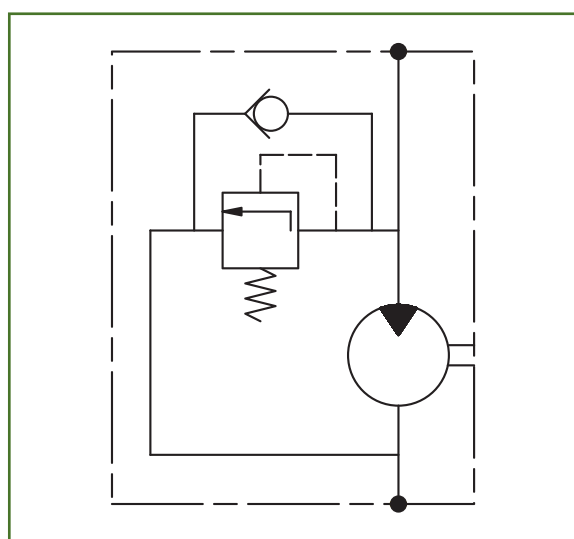
Schema idraulico Hydraulic circuit
